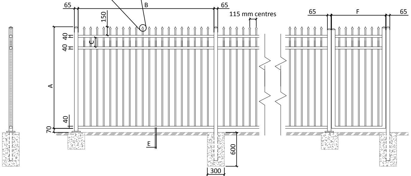
End View
