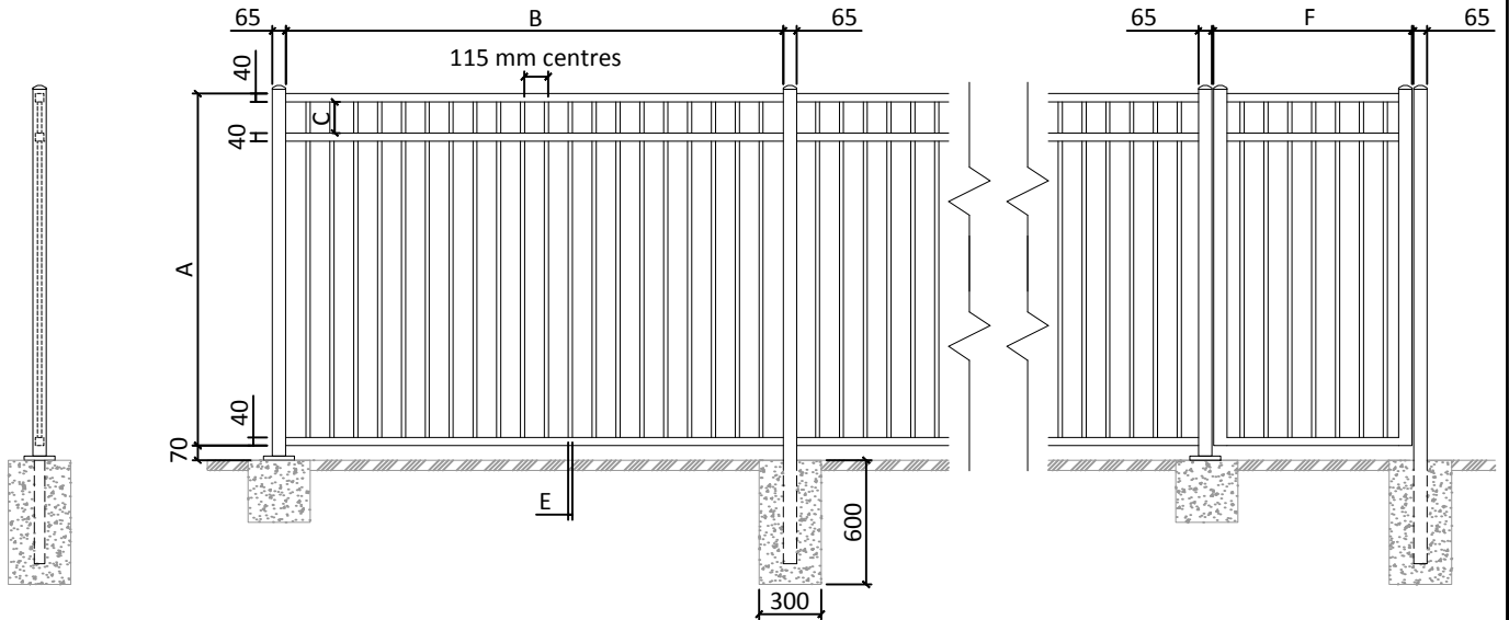
End View
