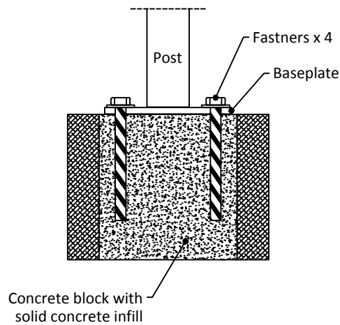
(c) To Concrete Block / Brick
