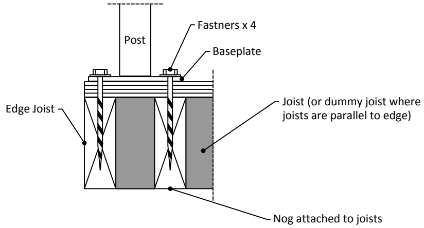
(a) To Timber:
