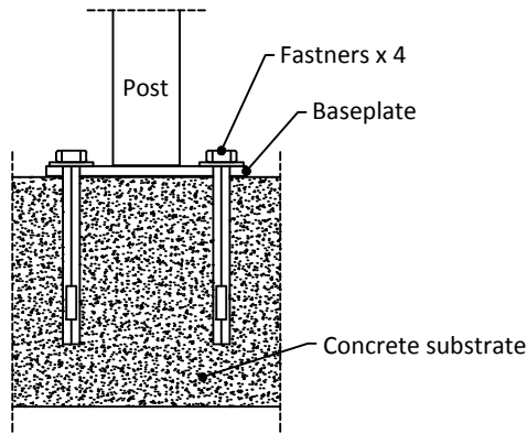
(b) To Concrete:
